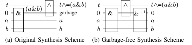
Fig. 2. SyReC synthesis for t \oplus = (a \odot b)
