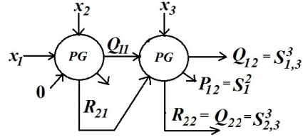
Fig. 5. Design for 3-inputs
