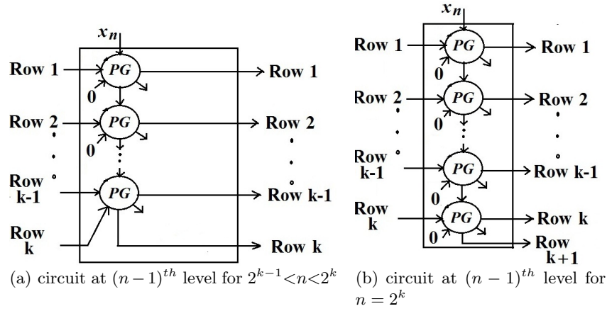
Fig. 7. The circuit structure at (n-1)^{th} level
