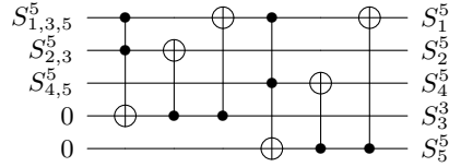
Fig. 12. EE modules appended at the end of the regular structure for 5 inputs
