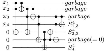
Fig. 9. Optimized design for 4-inputs
