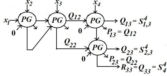
Fig. 6. Design for 4-inputs
